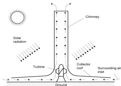
Fig.2. Solar chimney power configuration
