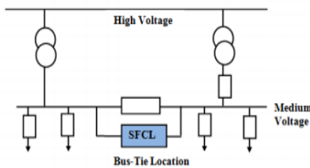
Fig. 5 SFCL in Bus-Tie Location
