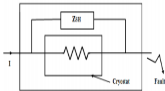
Fig.3 SFCL with Cooling System
