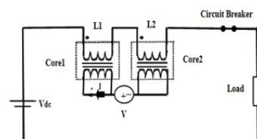
Fig.8 Inductive SFCL Circuit Diagram
