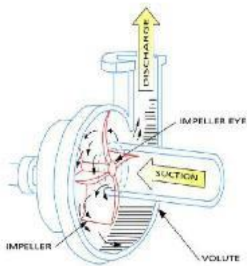
Fig.1. working principle of centrifugal pump
